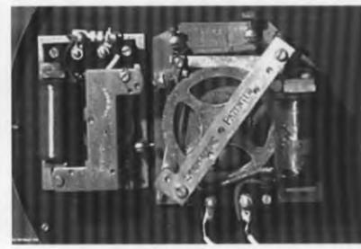
Slave dial mechanism. Each pulse from the C.P. advances a 120-tooth ratchet wheel carrying the minute hand by one tooth. These were normally imported from the UK or
