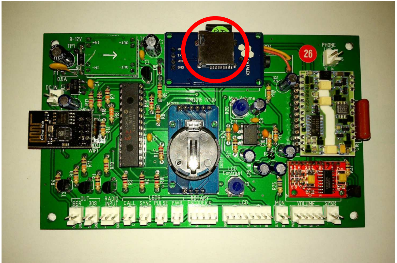
TIM 2015 interior view. You can see the microSD card projecting out of its silvery socket, ringed in red. Pushing it in, then pulling it out will release the card. If you use the Flexible Extension Cable Adapter, the connector plugs in where you see the microSD card in this photo.
