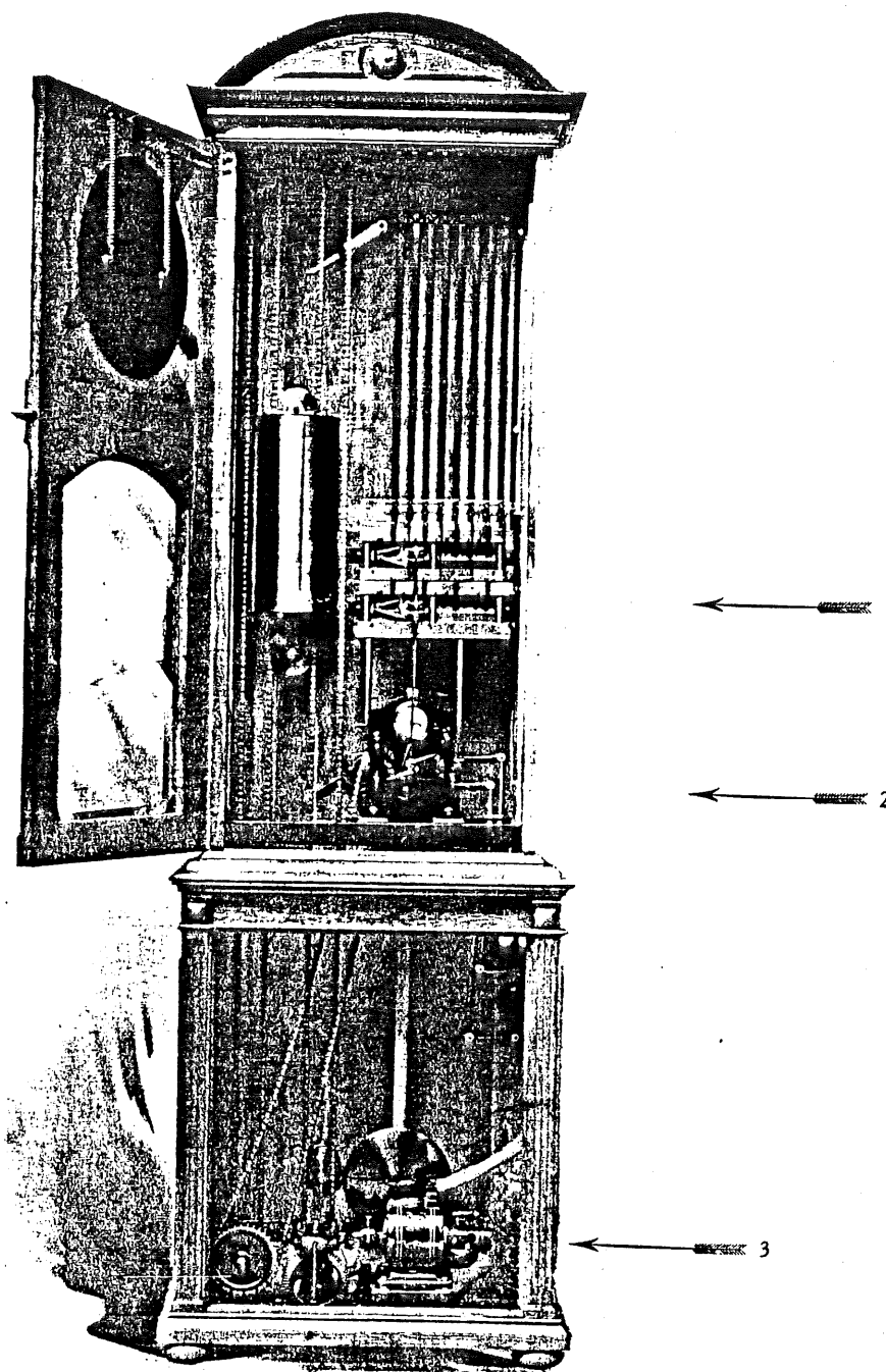
Apparatus as arranged in Master-clocks—Types f—i
