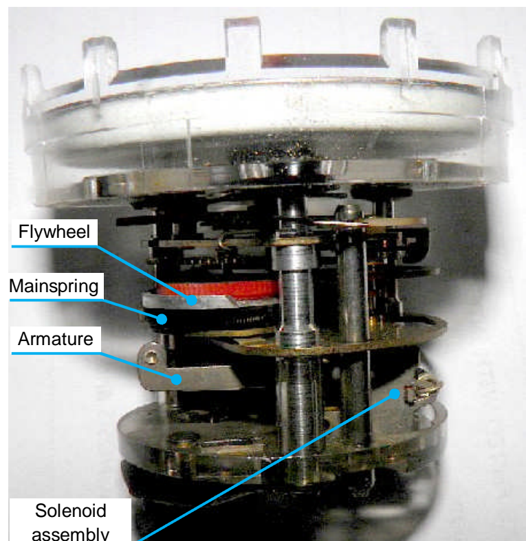
FIGURE 1.16: Another brand of clock. This electrically wound clock is branded "Borg". Photo shows similarity to the Kienzle electrically wound clock.
