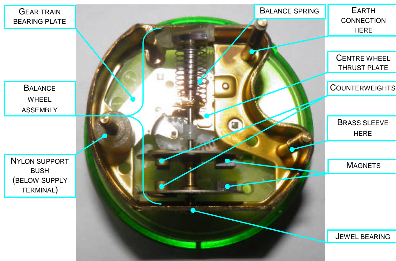
FIGURE 2.4: Balance and clock frame assemblies of a Kienzle transistorised clock. The clock has been removed from the case and only the circuit board removed in this view.
