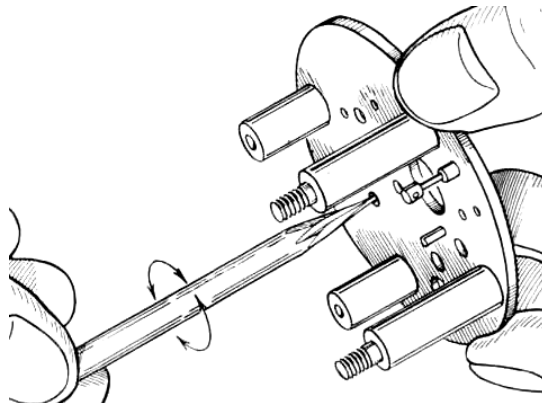
FIGURE.A.1: Pegging Pivot Holes
