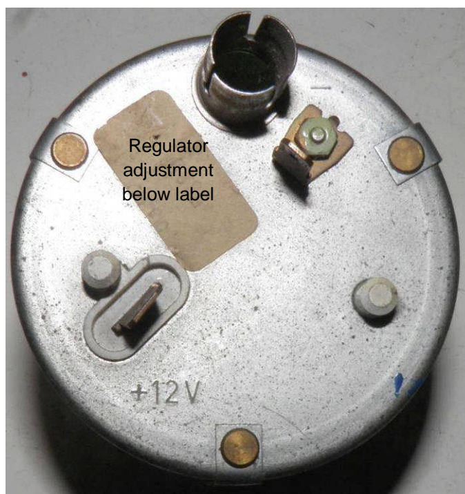
FIGURE 2.1: Showing the rear of the case prior to removal of the internal assemblies.
