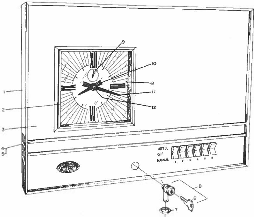
Door Panel Assembly and Trim Figure 1
