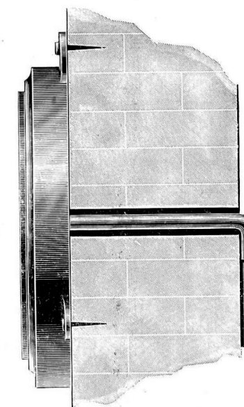
Fig. c 21. Sectional View Shewing Terminals led indoors.
