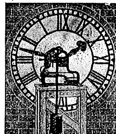
Waiting-Train Movement in a Clock Chamber behind an illuminated dial. Suitable for Turrets, Towers, Steeples, etc.
