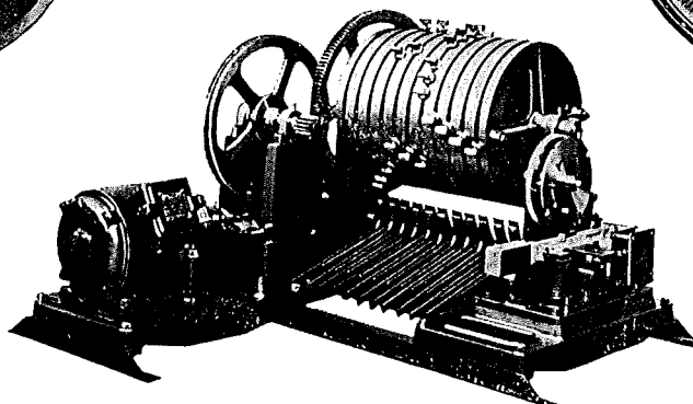
TYPICAL STRIKING, CHIMING AND TUNE MECHANISM.
