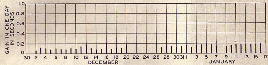
FIGURE 6 Daily rate of crystal clock against Naval Observatory time signals (corrected).
