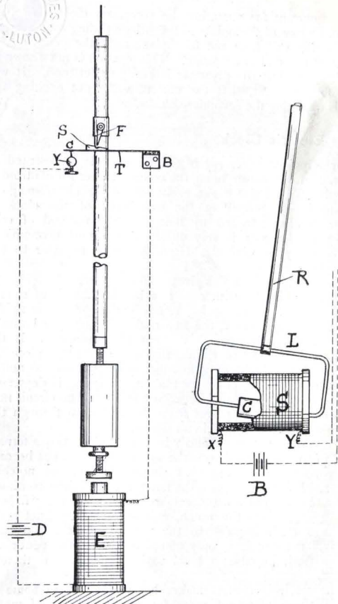
FIG. 3. Hipp's "Electric Pendulum." FIG. 3A. Wengelin's "Electric Pendulum."
