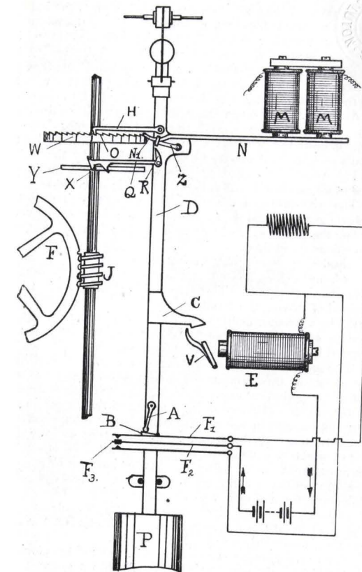
FIG. 58.—"Pulsynetic" Waiting Train Movement.
