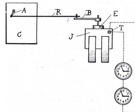
FIG. 66.—The "Magneta" Electric Clock System.
