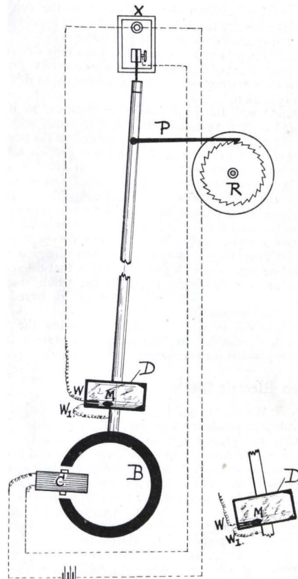
FIG. 8.—The Warren Electric Clock.
