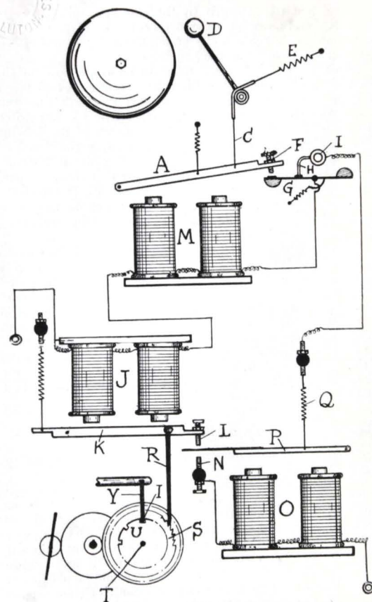
FIG. 52.—Parsons and Ball's Electrical Striking Gear.
