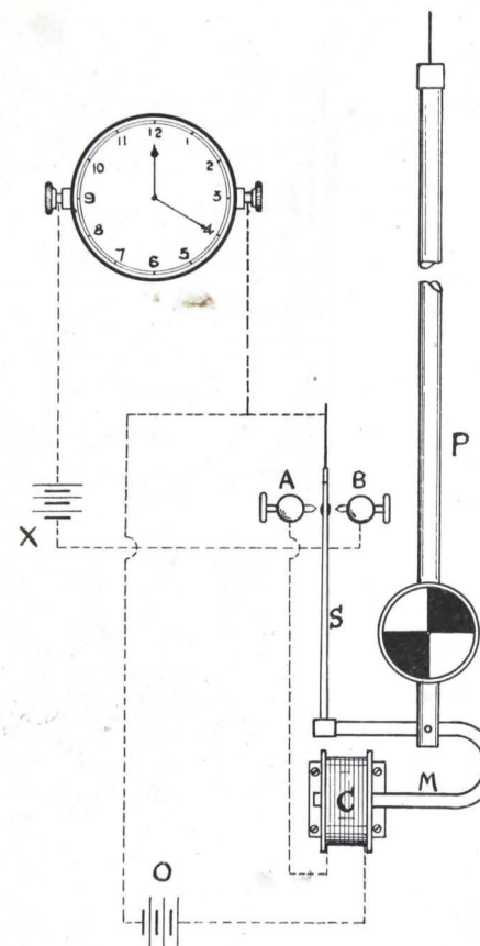
FIG. 6.—Féry's Electric Clock.
