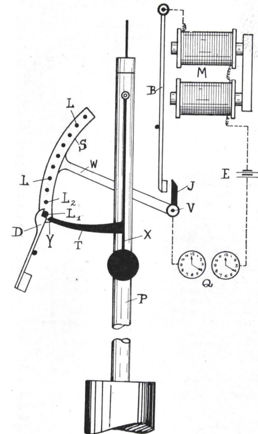
FIG. 32.—Walden's Electric Master Clock.
