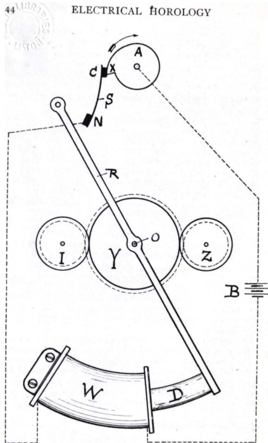
FIG. 16.—Wengelin's Winding Gear.
