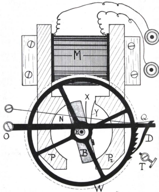
FIG. 41.—Murday's Electric Secondary Clock.
