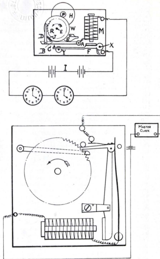
FIGS. 21 and 21A. —Hope-Jones and Bowell's Electrically Wound Clock.
