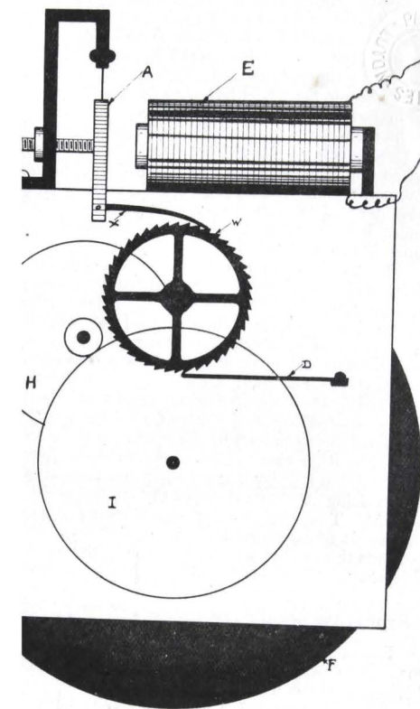
FIG. 34.—Bain's Electric Secondary Clock.
