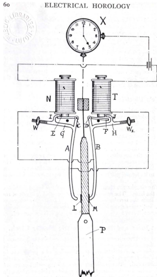
FIG. 24.—Hope-Jones and Bowell's Electric Master Clock.
