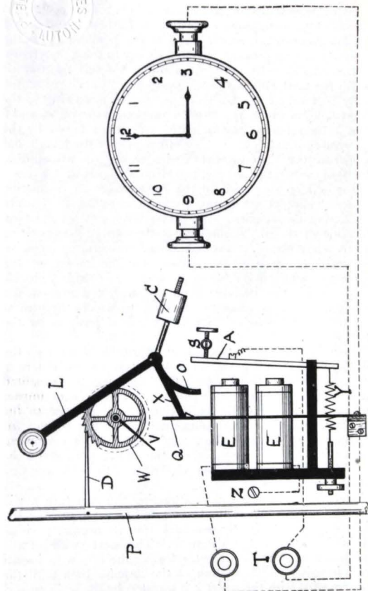
FIG. 23.—Stelje's Electric Master Clock.
