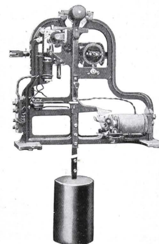
FIG. 59.—The "Pulsynetic" Waiting Train Movement.
