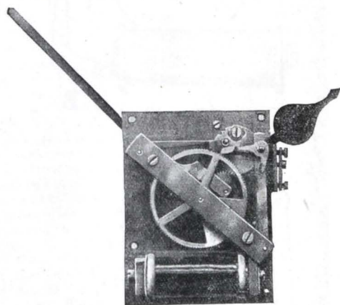
FIG. 44.—The "Pulsynetic" Impulse Clock.
