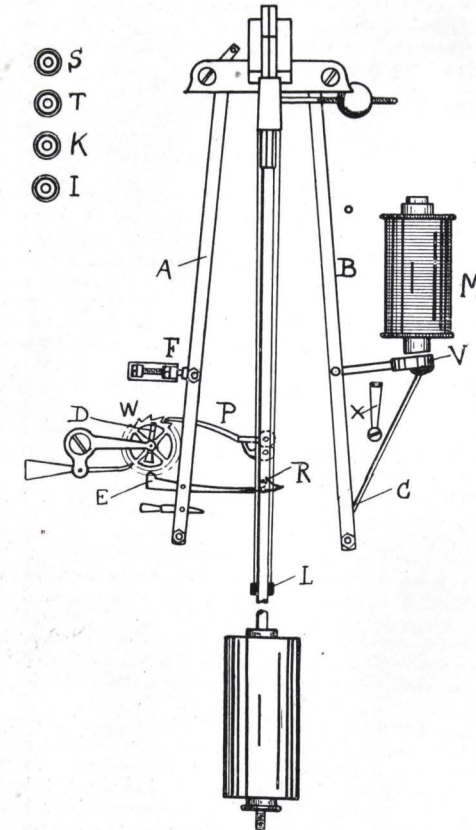
FIG. 25.—Electric Master Clock for "The Standard Time" System.
