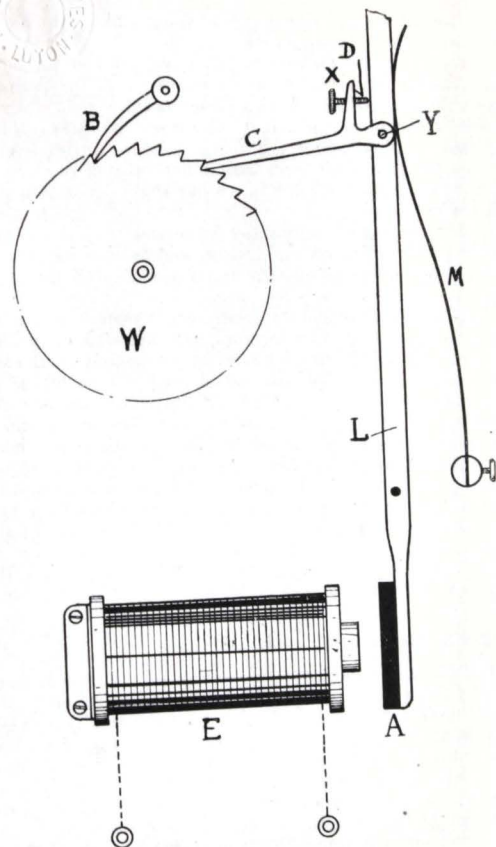
FIG. 49.—Parker's Electric Secondary Clock.
