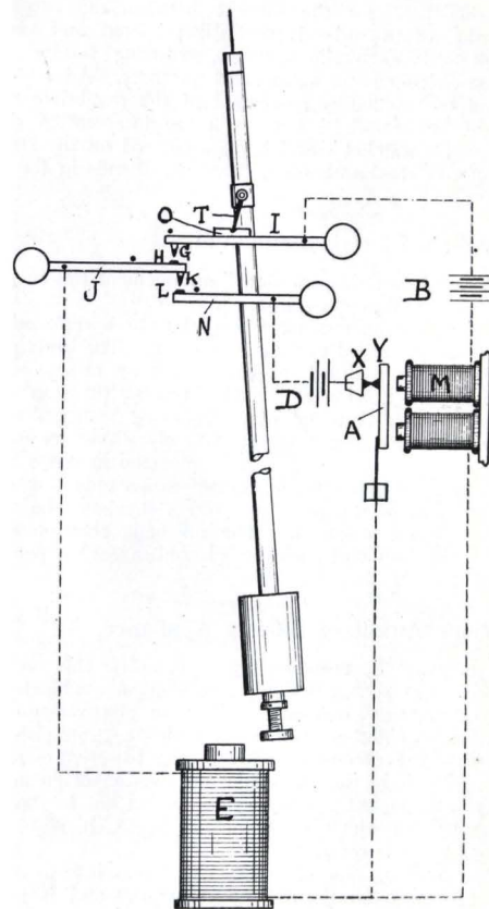
FIG. 9.—Webber's Auxiliary Battery Appliance.
