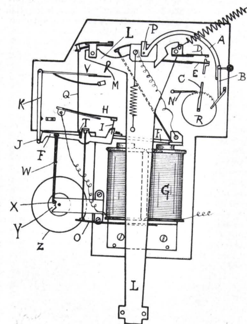
FIG. 26.—The Lowne Electric Master Clock.
