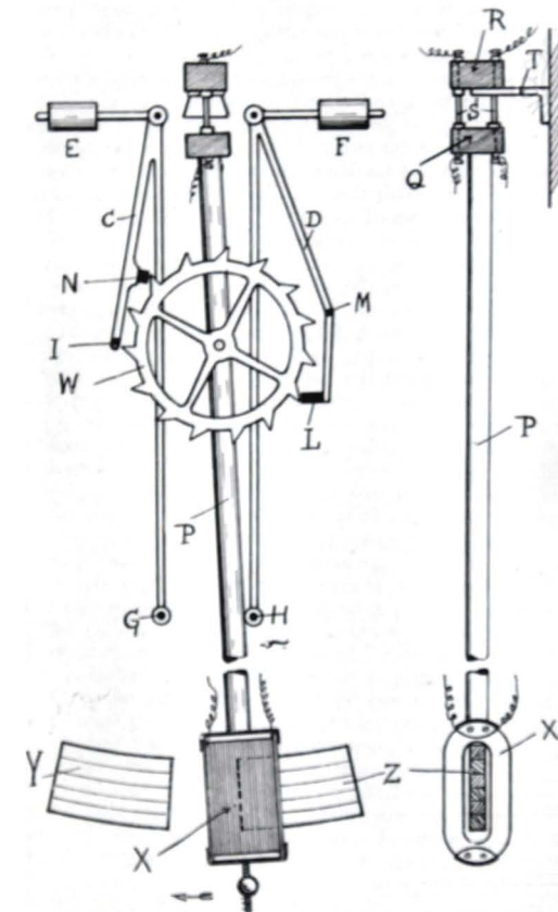
FIG. 12.—Ritchie's Electric Clock.
