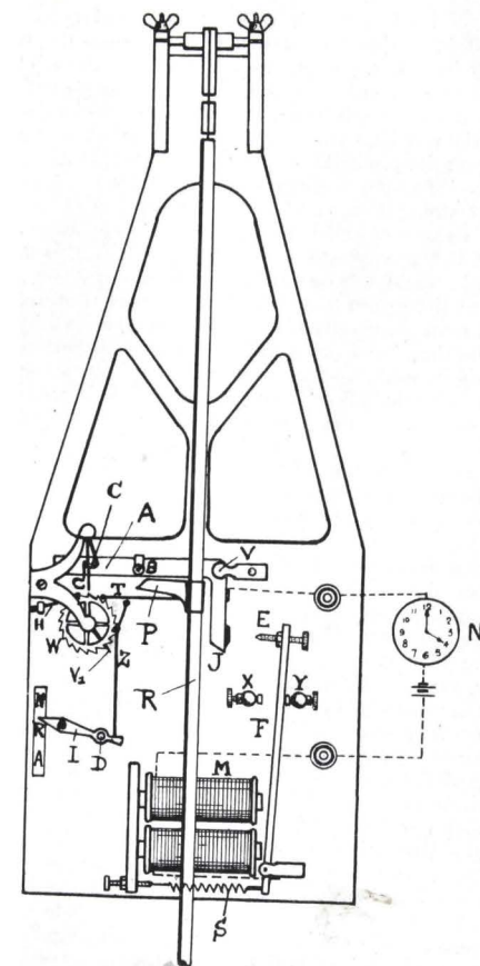
FIG. 27.—The "Synchronome" Electric Master Clock.
