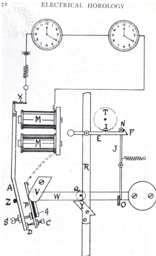
FIG. 29.—The "Pulsynetic" Electric Master Clock.
