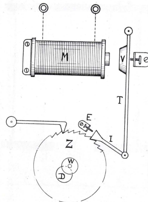
FIG. 36.—Stelje's Electric Secondary Clock.
