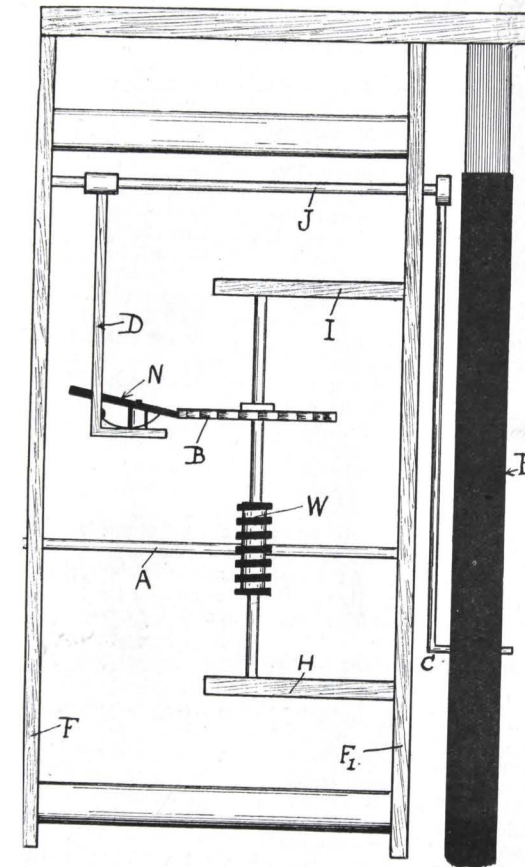
FIG. 4.—Early Form of Electric Turret Clock.
