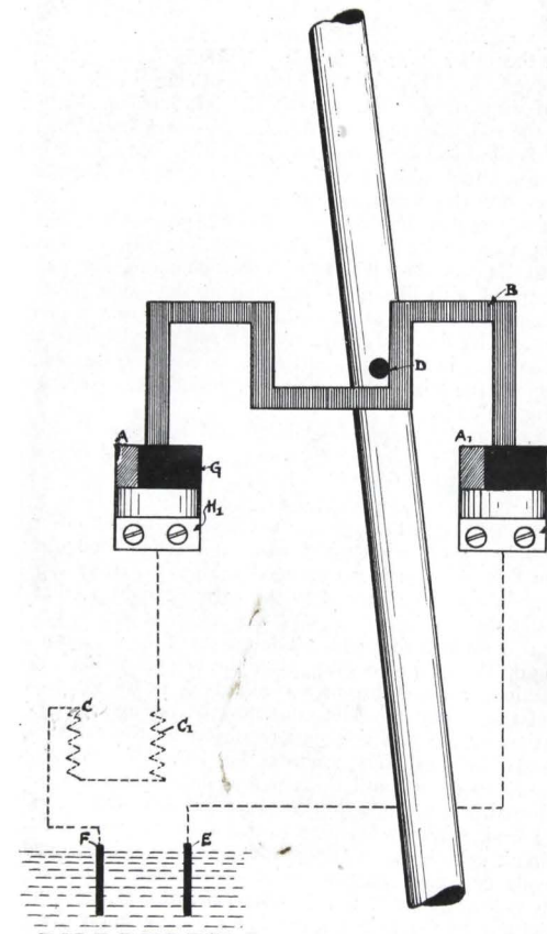
FIG. 2.—Bain's Electric "Break."
