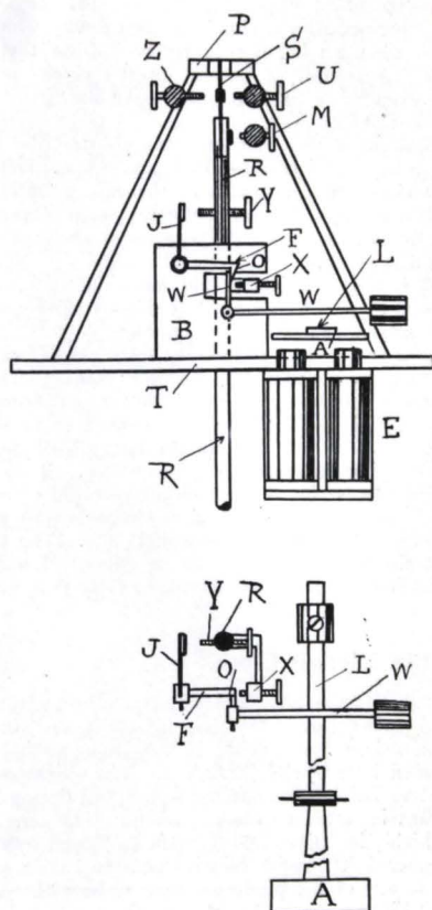
FIG. 22.—Shepherd's Electric Clock.
