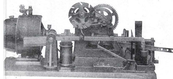
FIG. 54.—"Pulsynetic" Motor-Driven Striking Mechanism.
