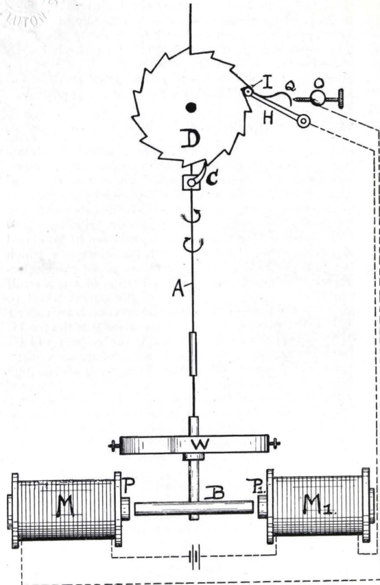
FIG. 62.—Reid's Electrically Driven Balance-Wheel Clock.
