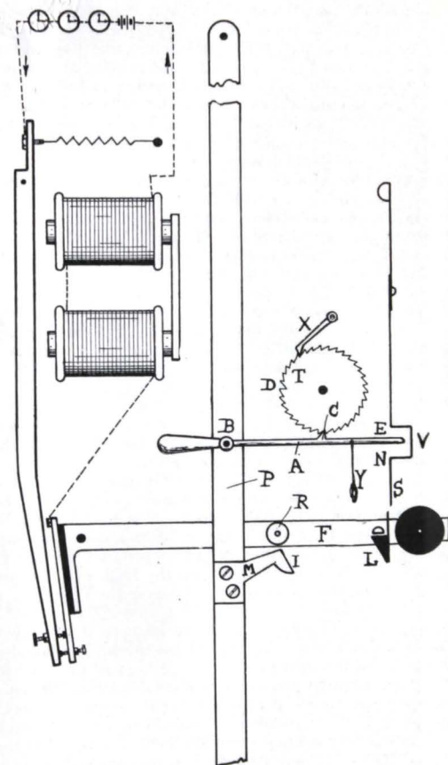
FIG. 30.—Standard "Pulsynetic" Electric Master Clock.
