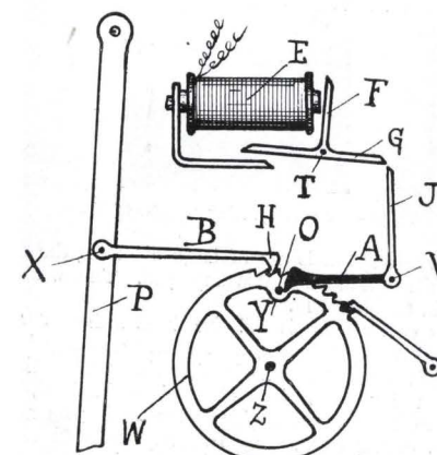
FIG. 43.—"Pulsynetic" Waiting Train Movement.
