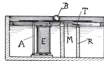
FIG. 65.—Boulton's Electric Clock Controller.
