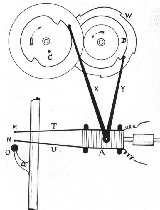
FIG. 33.—Murday's Electric Transmitter.
