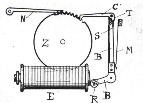
FIG. 42.—The "Pulsynetic" Electric Impulse Clock.
