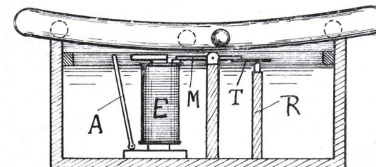
FIG. 64.—Boulton's Electric Clock Controller.
