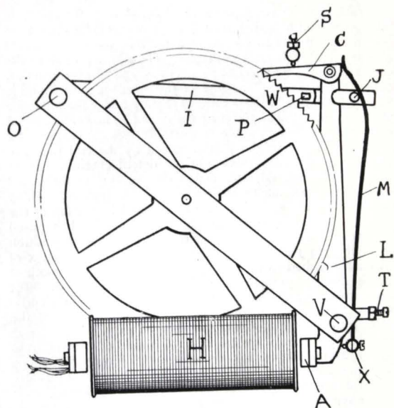
FIG. 40.—The "Synchronome" Electric Secondary Clock.
