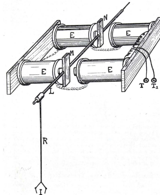
FIG. 14.—Electro-Mechanism of the Brequet Electric Clock.
