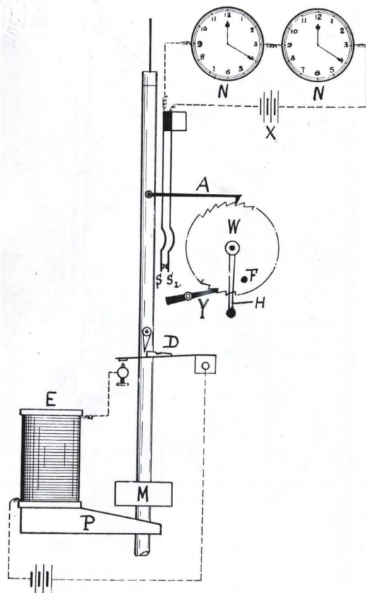
FIG. 7.—The Swift Electric Clock.
