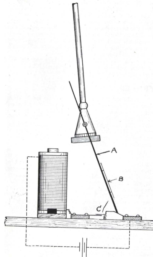
FIG. 5.—Lemoine's Electric Clock.
