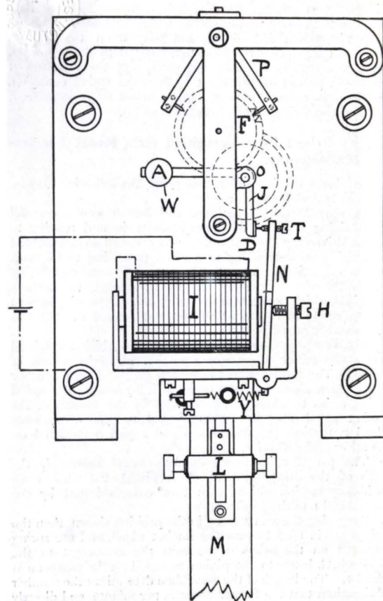
FIG. 19.—Clock Driven by Electrically Raised Weighted Arm.
