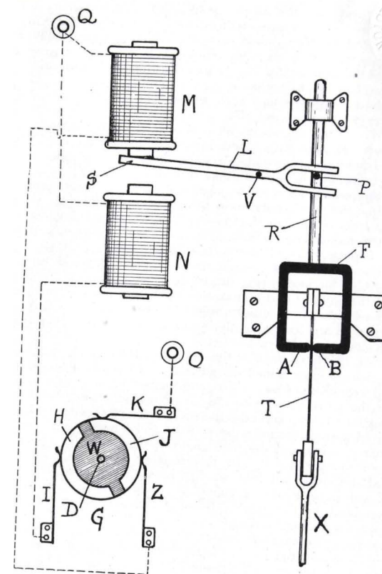
FIG. 60.—Hope-Jones and Bowell's Synchronising Mechanism.
