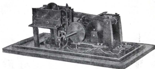
FIG. 55.—"Pulsynetic" Waiting Train Driven Striking Mechanism.
