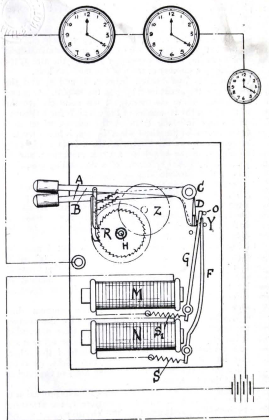
FIG. 20.—Electric Clock with Two Weighted Arms.
