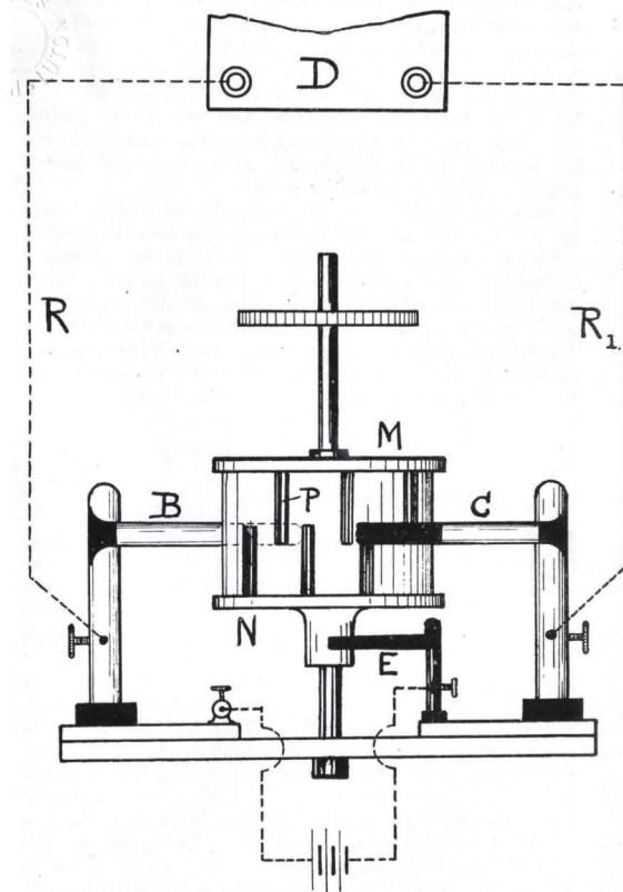
FIG. 13.—Brequet's Lantern Electric Clock.
