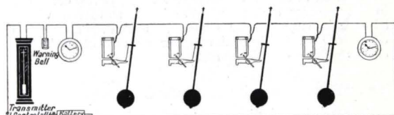
FIG. 45.—The "Reflex" Pendulum Control.
