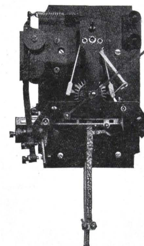
FIG. 31. The "Thornbridge" Transmitter.
