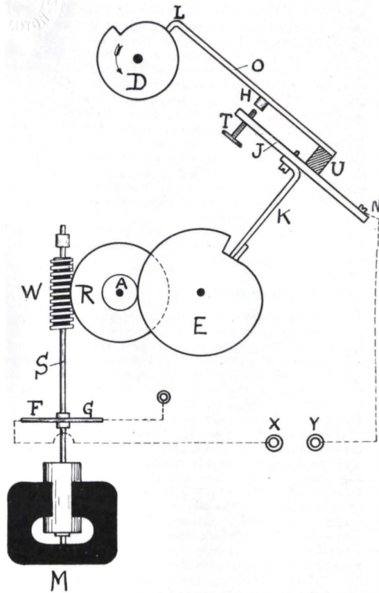
FIG. 17.—Steiger's Winding Gear.
