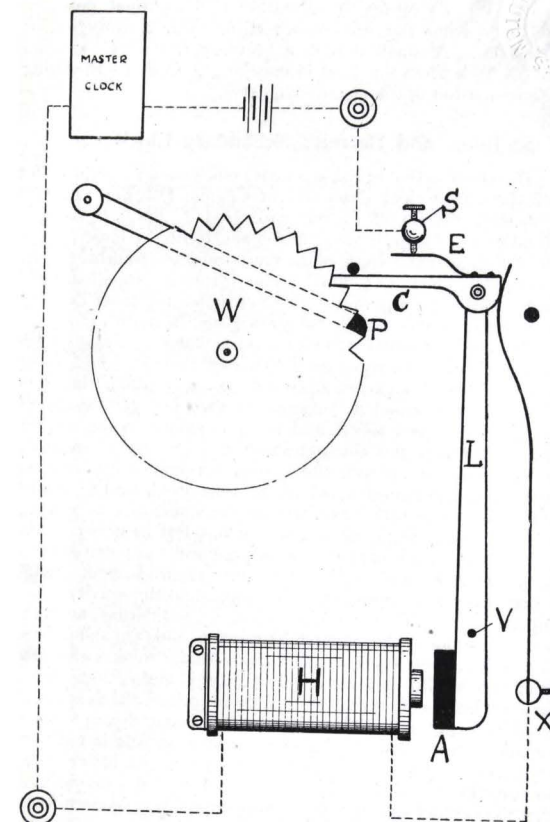
FIG. 49A.—Hope-Jones and Bowell's Electric Secondary Clock.
