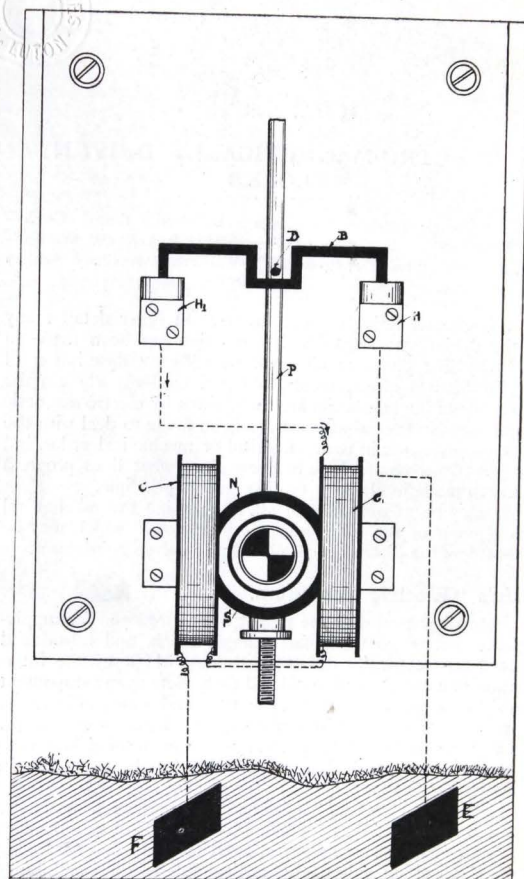
FIG. 1.—Bain's "Electric Pendulum."
