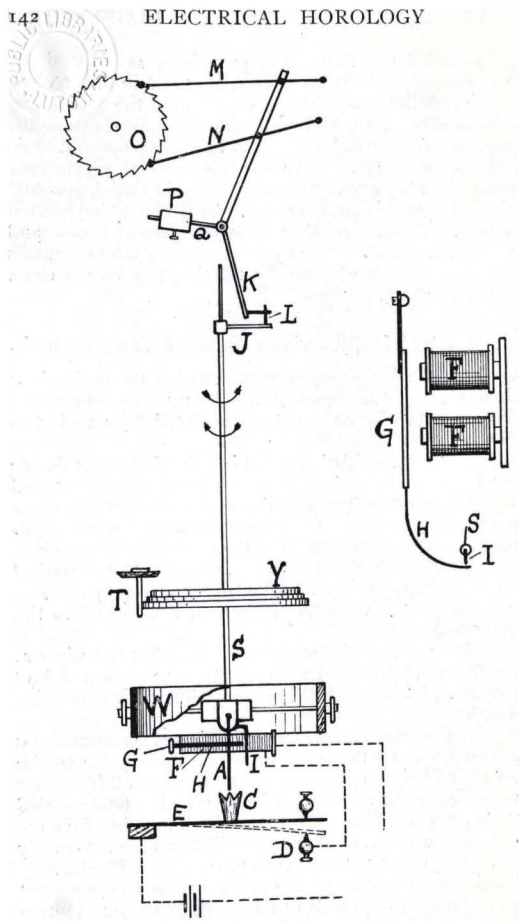
FIG. 61.—Murday's Electrically Driven Balance-Wheel Clock.
