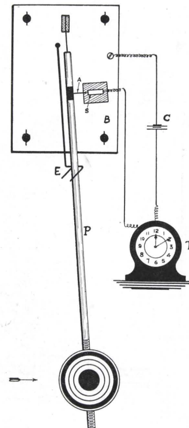
FIG. 10.—Bain's Electric Transmitter.
