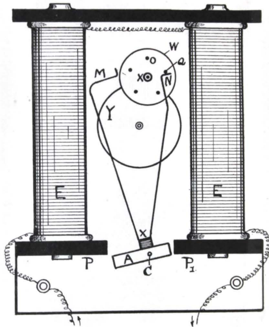
FIG. 37.—The Swift Electric Secondary Clock.
